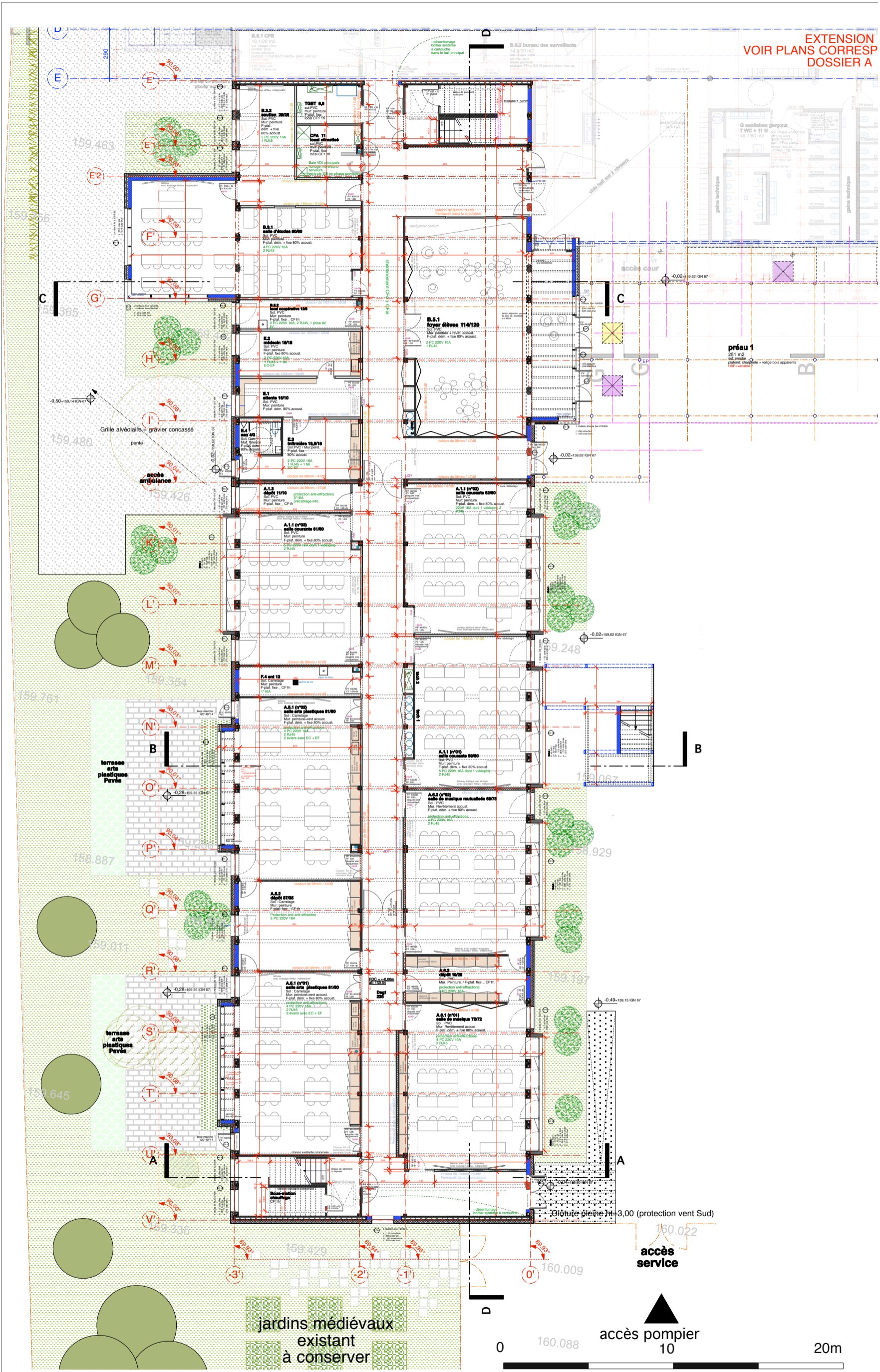
PLAN Rdc _ EXISTANT PHASE APD
